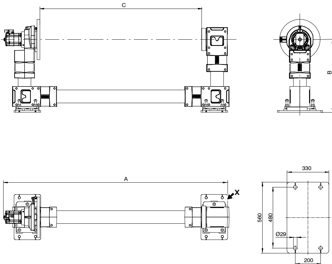
“X” Lochbild Maschinengestellbefestigung Hole pattern for machine frame mounting
